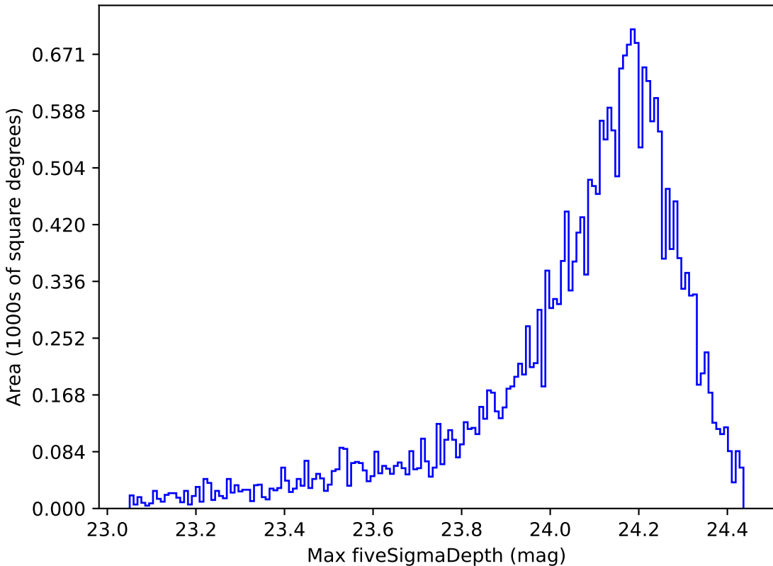
too_elab_r64_d3_gz_v3.4_10yrs Yr 1 i band: Max fiveSigmaDepth
