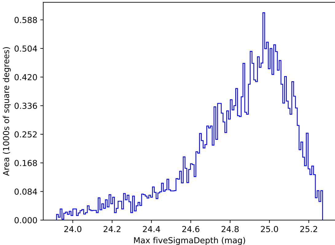
too_elab_r64_d3_gz_v3.4_10yrs Yr 1 g band: Max fiveSigmaDepth
