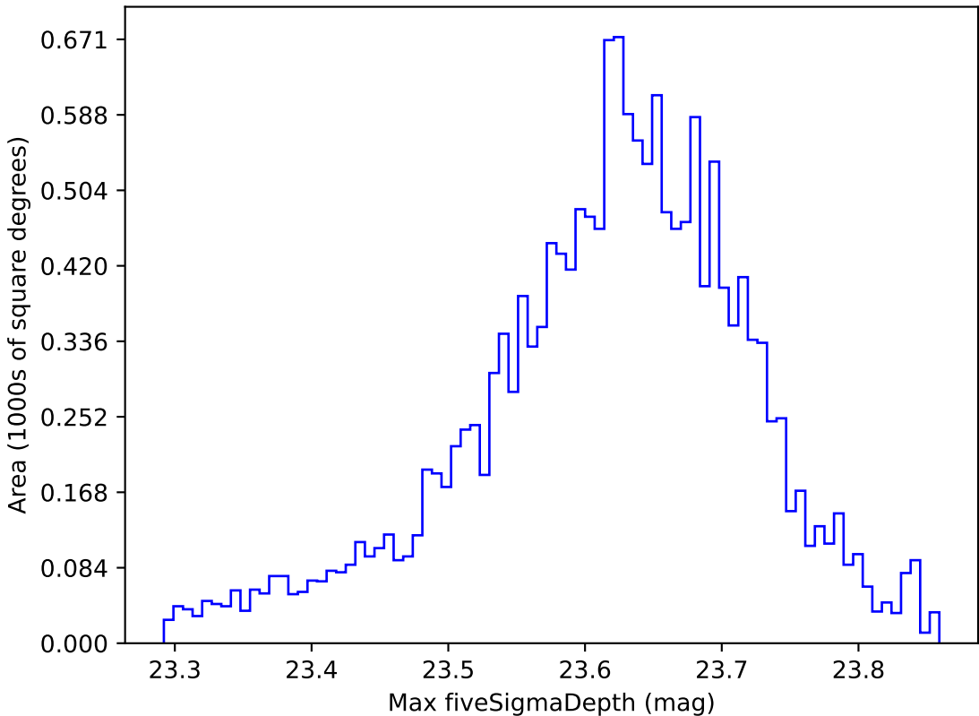
too_elab_r64_d3_gz_v3.4_10yrs WFD z band: Max fiveSigmaDepth
