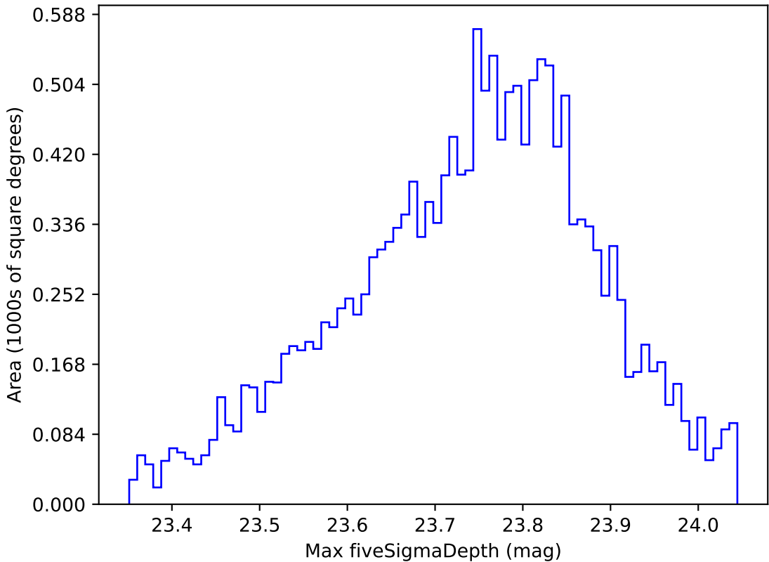
too_elab_r64_d3_gz_v3.4_10yrs WFD u band: Max fiveSigmaDepth
