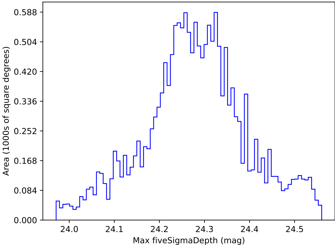
too_elab_r64_d3_gz_v3.4_10yrs WFD i band: Max fiveSigmaDepth
