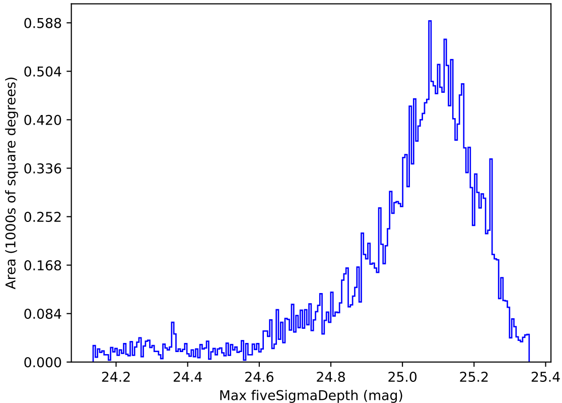
too_elab_r64_d3_gz_v3.4_10yrs All sky g band: Max fiveSigmaDepth
