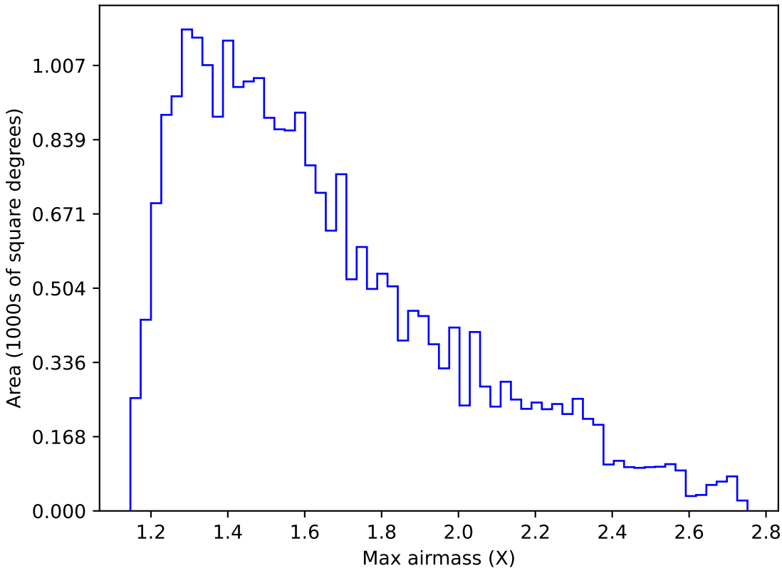
too_elab_r64_d3_gz_v3.4_10yrs Yr 1 z band: Max airmass
