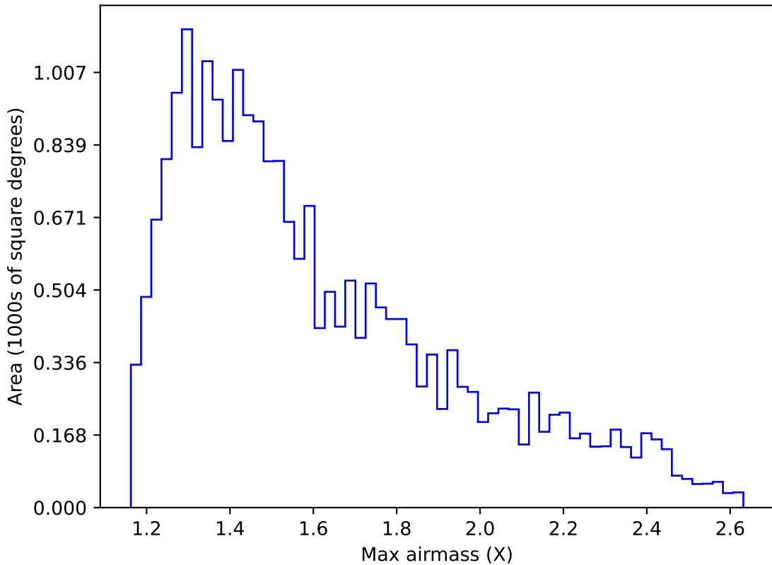
too_elab_r64_d3_gz_v3.4_10yrs Yr 1 y band: Max airmass
