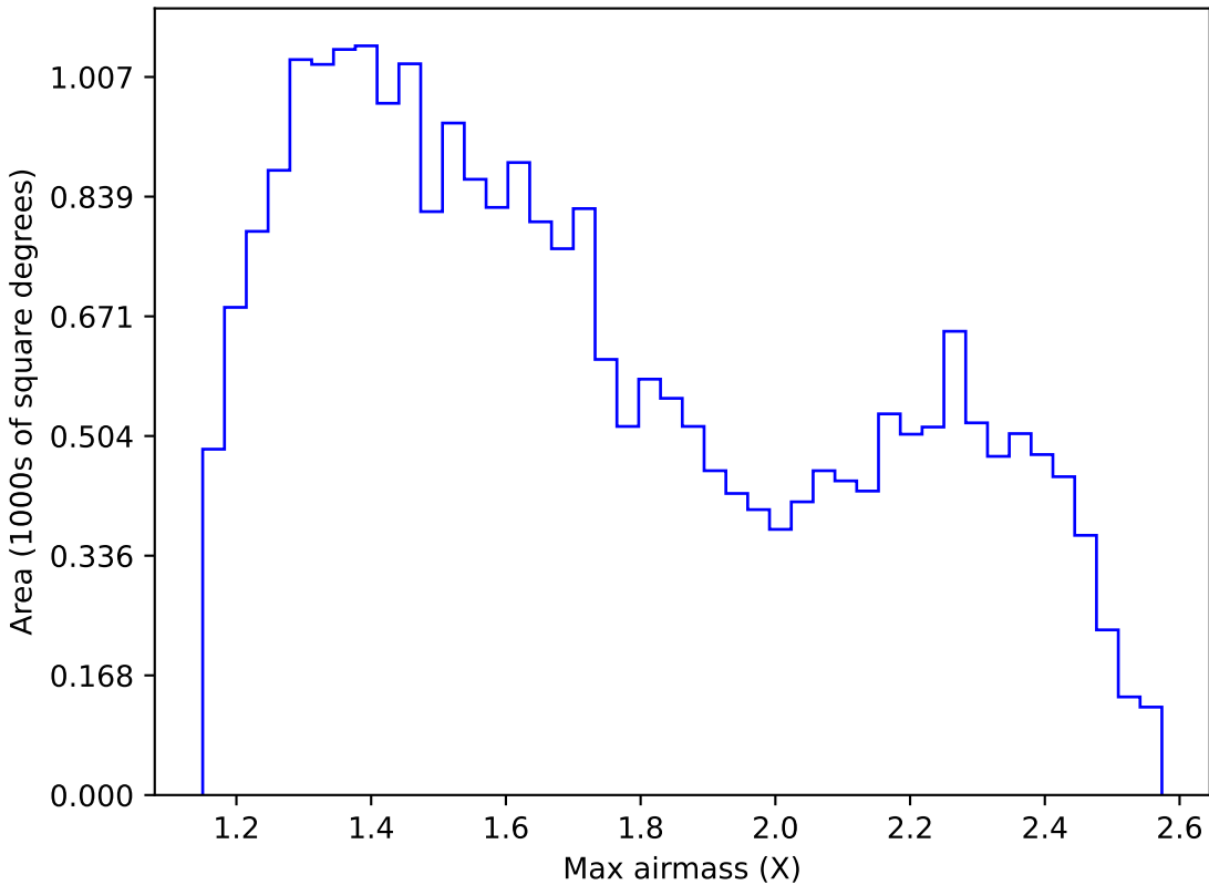
too_elab_r64_d3_gz_v3.4_10yrs Yr 1 r band: Max airmass
