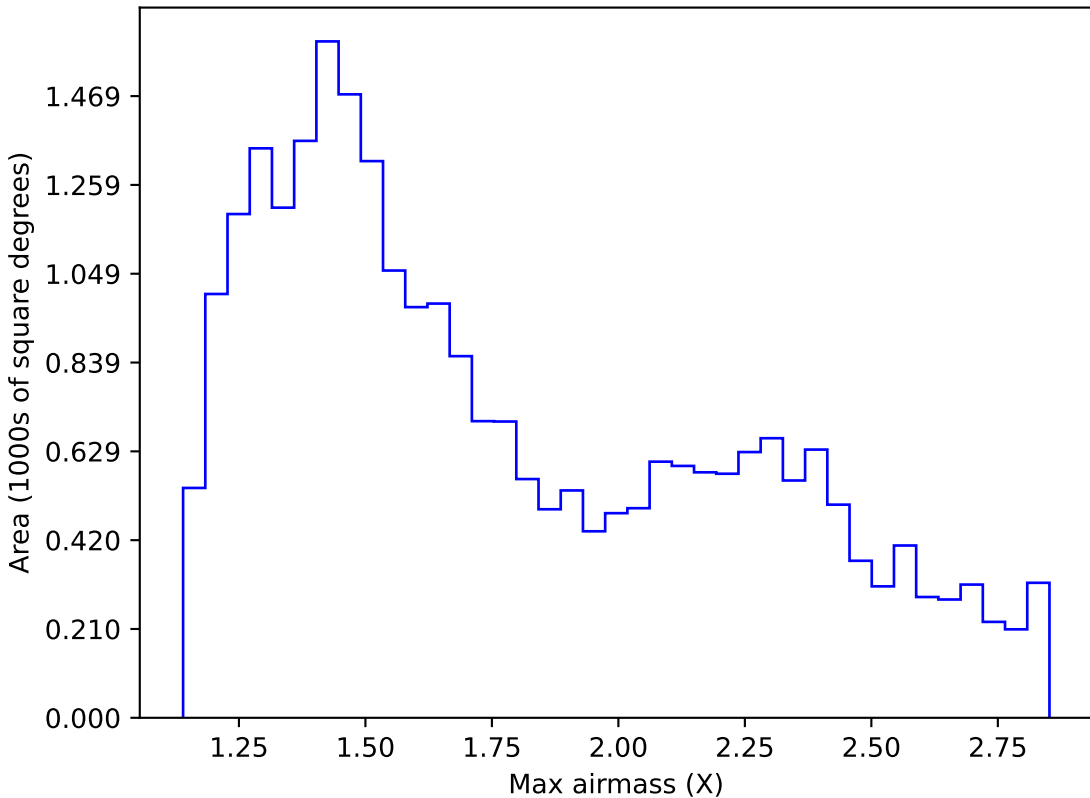
too_elab_r64_d3_gz_v3.4_10yrs Yr 1 i band: Max airmass
