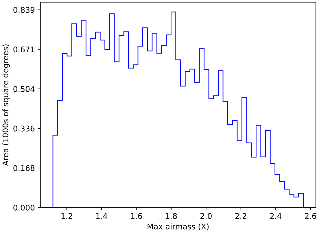
too_elab_r64_d3_gz_v3.4_10yrs Yr 1 g band: Max airmass
