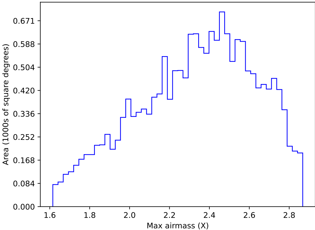
too_elab_r64_d3_gz_v3.4_10yrs WFD y band: Max airmass
