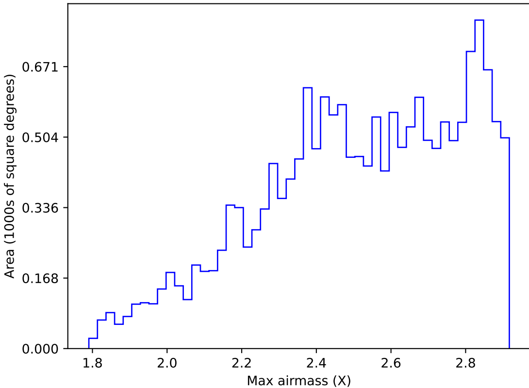
too_elab_r64_d3_gz_v3.4_10yrs WFD i band: Max airmass
