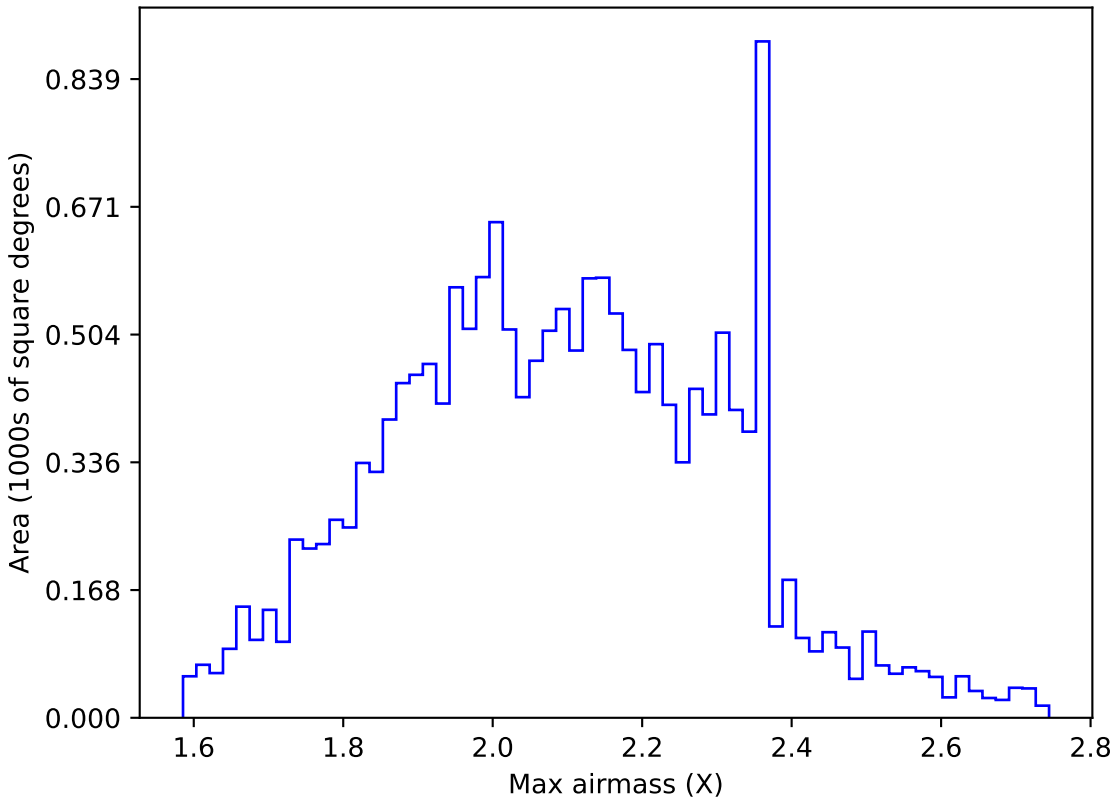
too_elab_r64_d3_gz_v3.4_10yrs WFD g band: Max airmass
