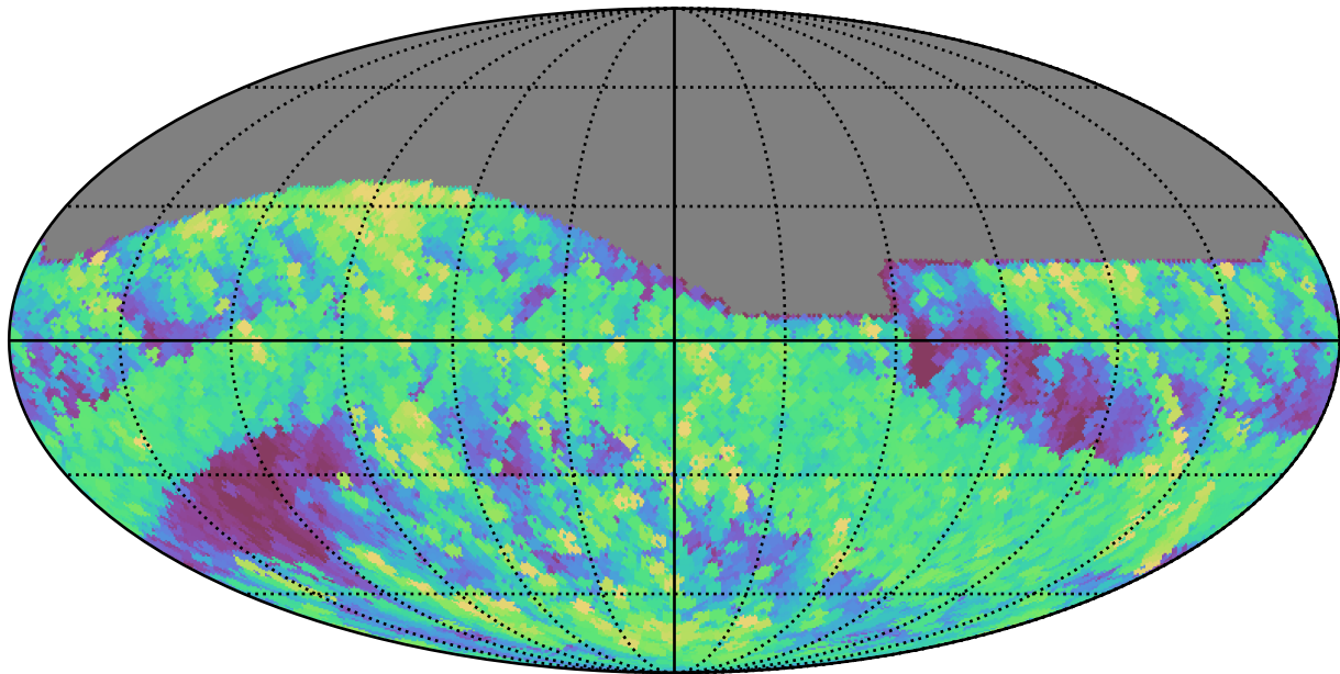
too_elab_r64_d3_gz_v3.4_10yrs All sky r band: Max airmass
