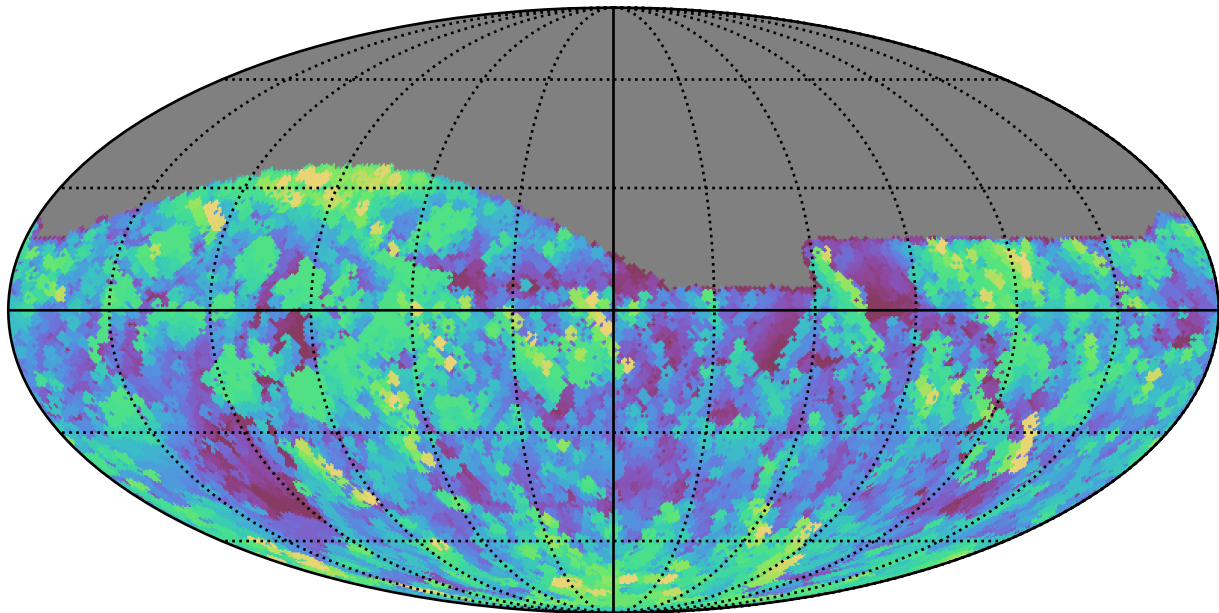
too_elab_r64_d3_gz_v3.4_10yrs All sky g band: Max airmass
