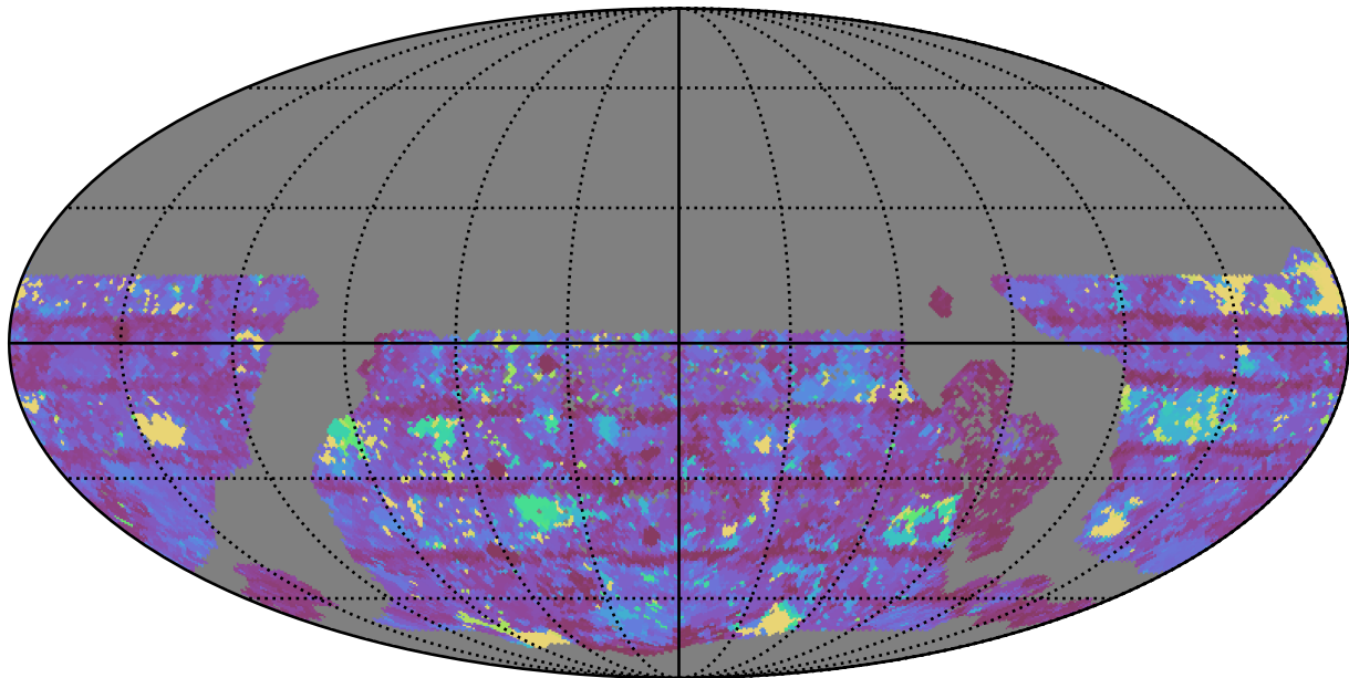
too_elab_r64_d3_gz_v3.4_10yrs WFD z band: Max Inter-Night Gap
