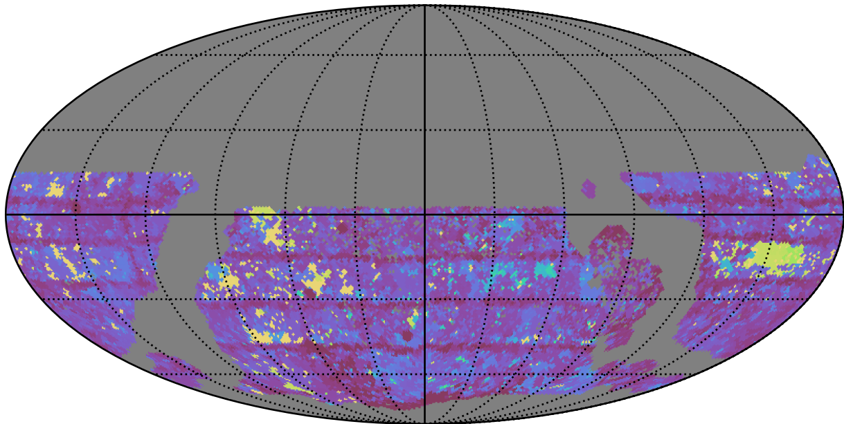
too_elab_r64_d3_gz_v3.4_10yrs WFD y band: Max Inter-Night Gap
