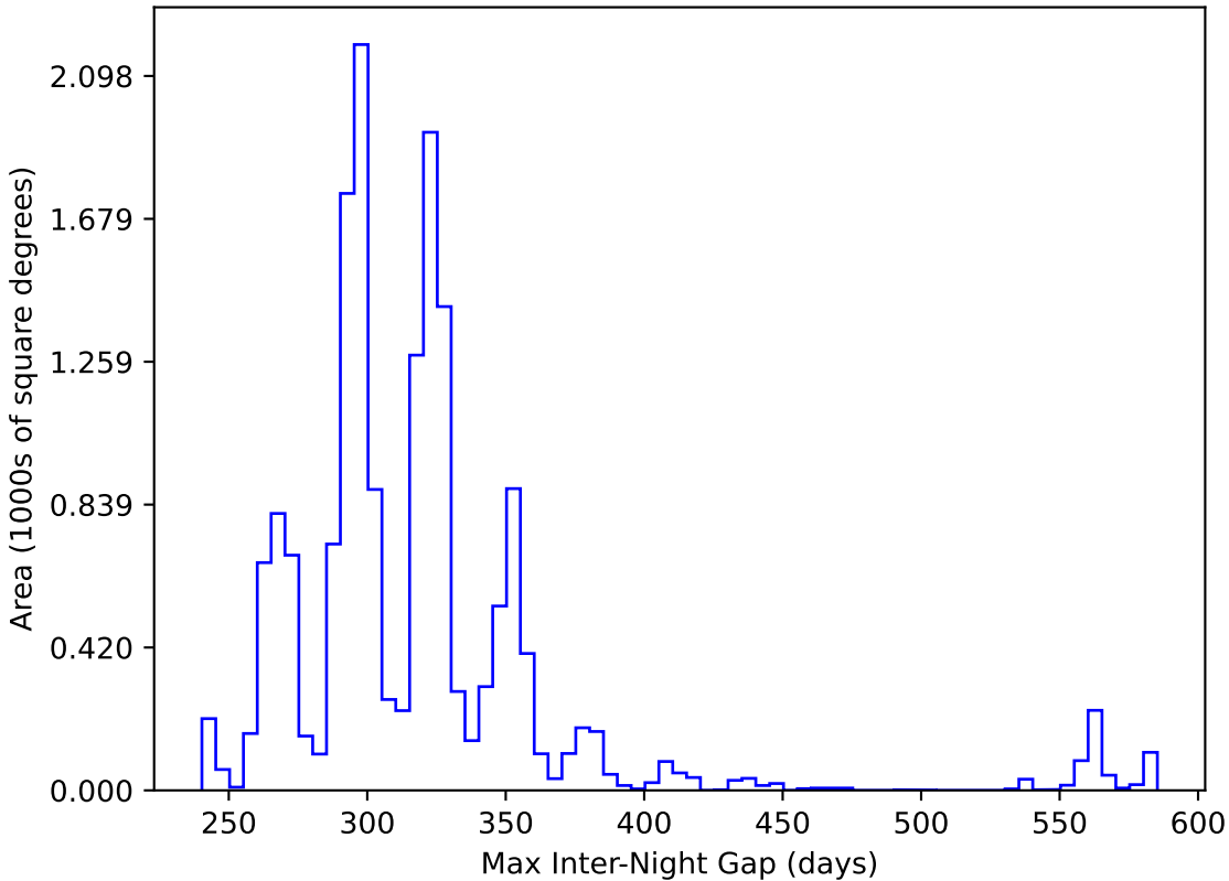
too_elab_r64_d3_gz_v3.4_10yrs WFD y band: Max Inter-Night Gap
