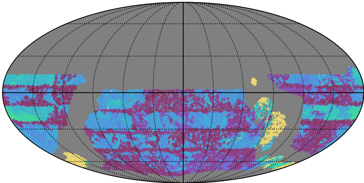
too_elab_r64_d3_gz_v3.4_10yrs WFD u band: Max Inter-Night Gap
