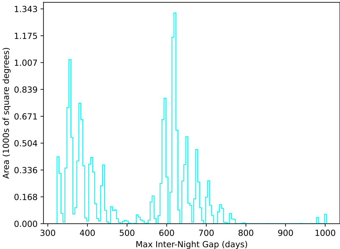
too_elab_r64_d3_gz_v3.4_10yrs WFD u band: Max Inter-Night Gap
