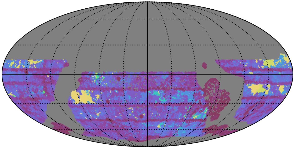
too_elab_r64_d3_gz_v3.4_10yrs WFD r band: Max Inter-Night Gap
