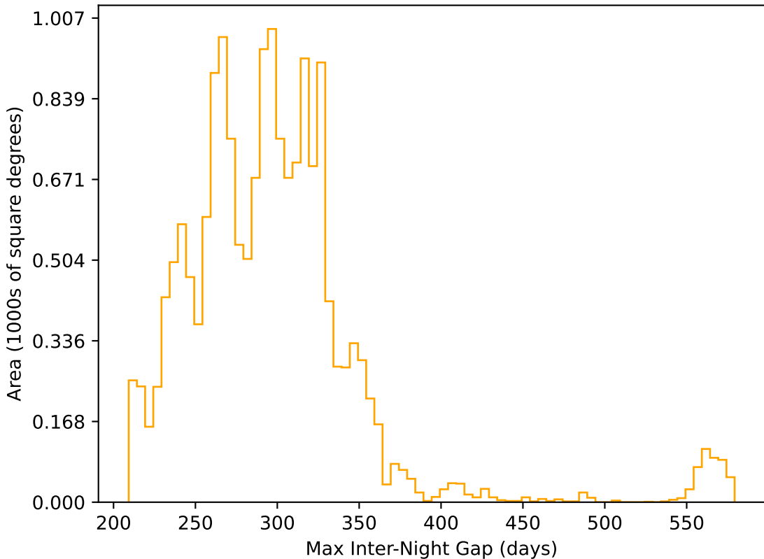
too_elab_r64_d3_gz_v3.4_10yrs WFD r band: Max Inter-Night Gap
