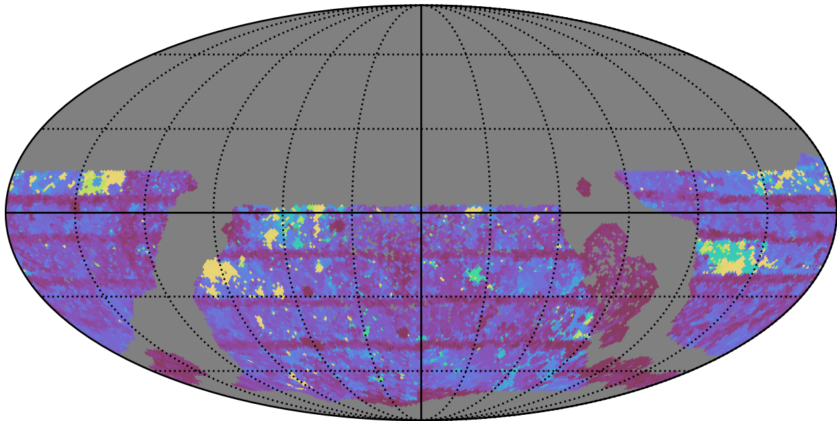
too_elab_r64_d3_gz_v3.4_10yrs WFD i band: Max Inter-Night Gap
