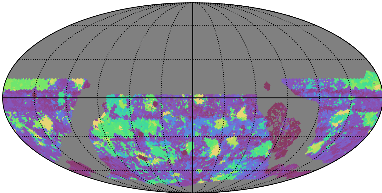
too_elab_r64_d3_gz_v3.4_10yrs WFD g band: Max Inter-Night Gap
