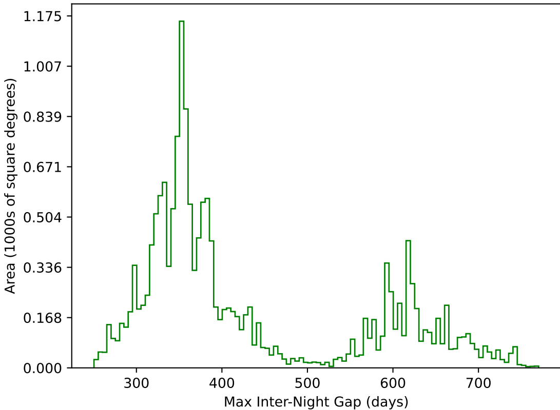
too_elab_r64_d3_gz_v3.4_10yrs WFD g band: Max Inter-Night Gap
