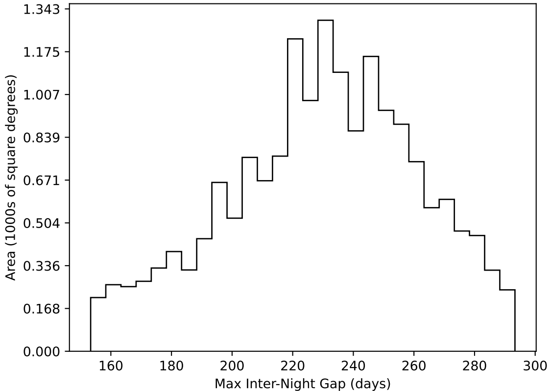
too_elab_r64_d3_gz_v3.4_10yrs WFD all bands: Max Inter-Night Gap
