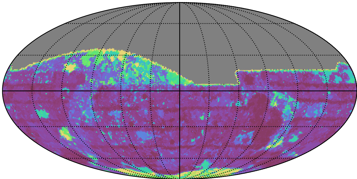
too_elab_r64_d3_gz_v3.4_10yrs All sky z band: Max Inter-Night Gap
