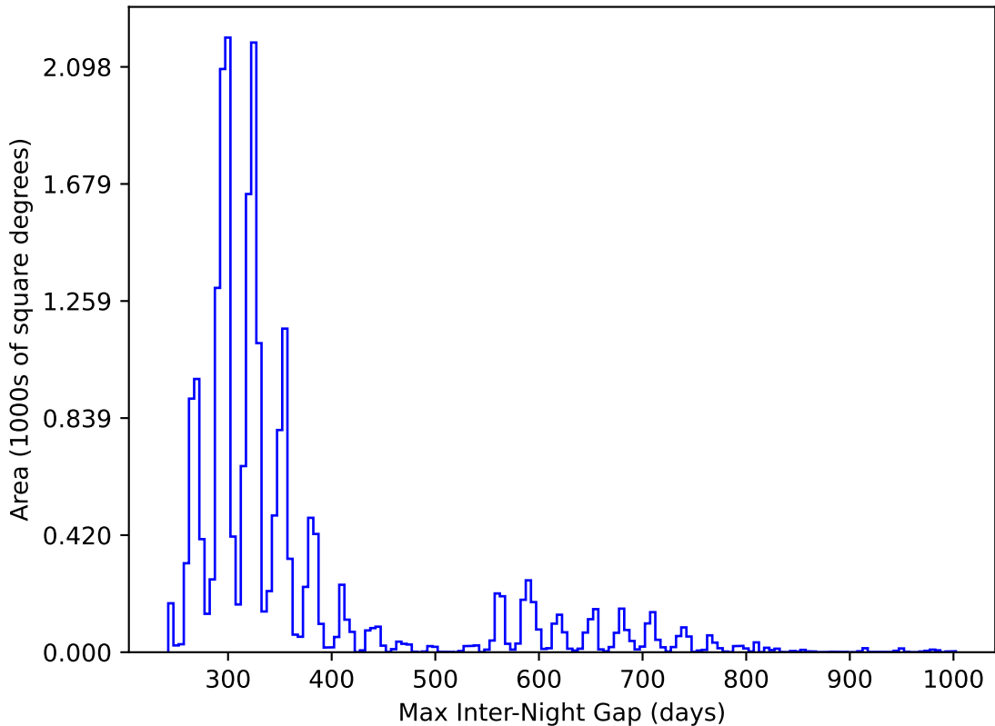
too_elab_r64_d3_gz_v3.4_10yrs All sky y band: Max Inter-Night Gap
