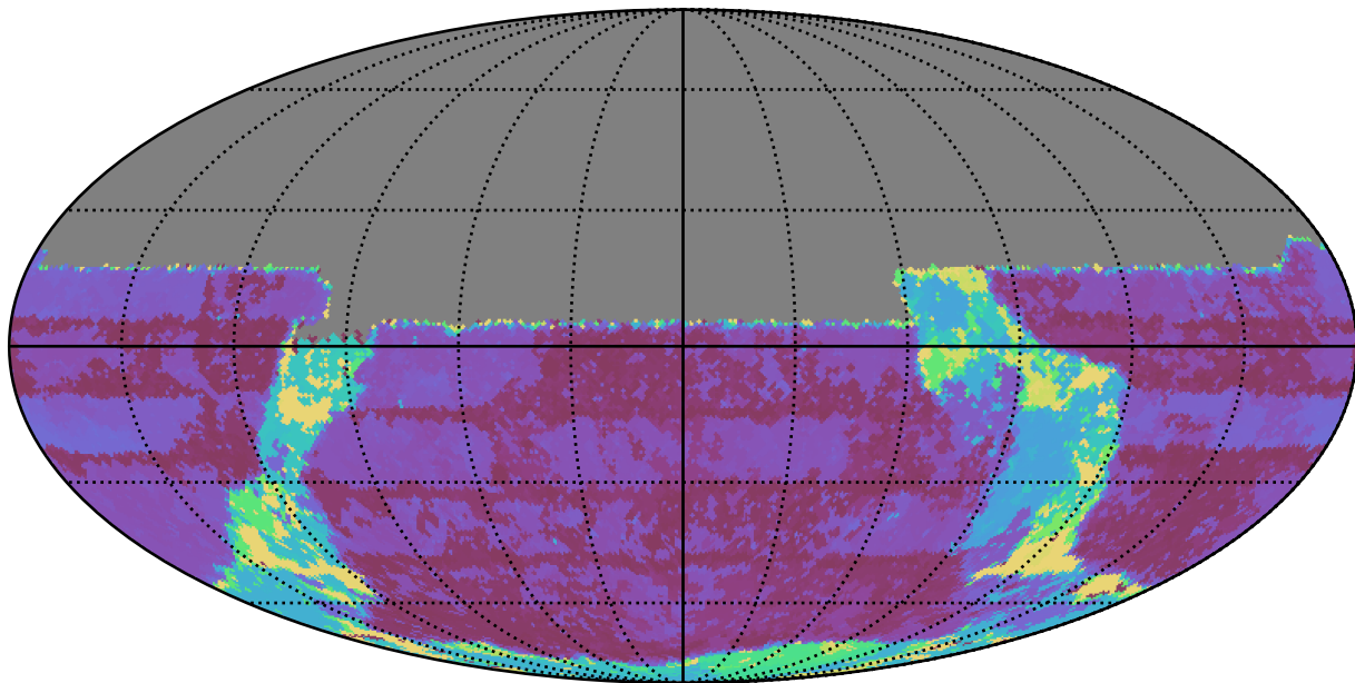
too_elab_r64_d3_gz_v3.4_10yrs All sky u band: Max Inter-Night Gap
