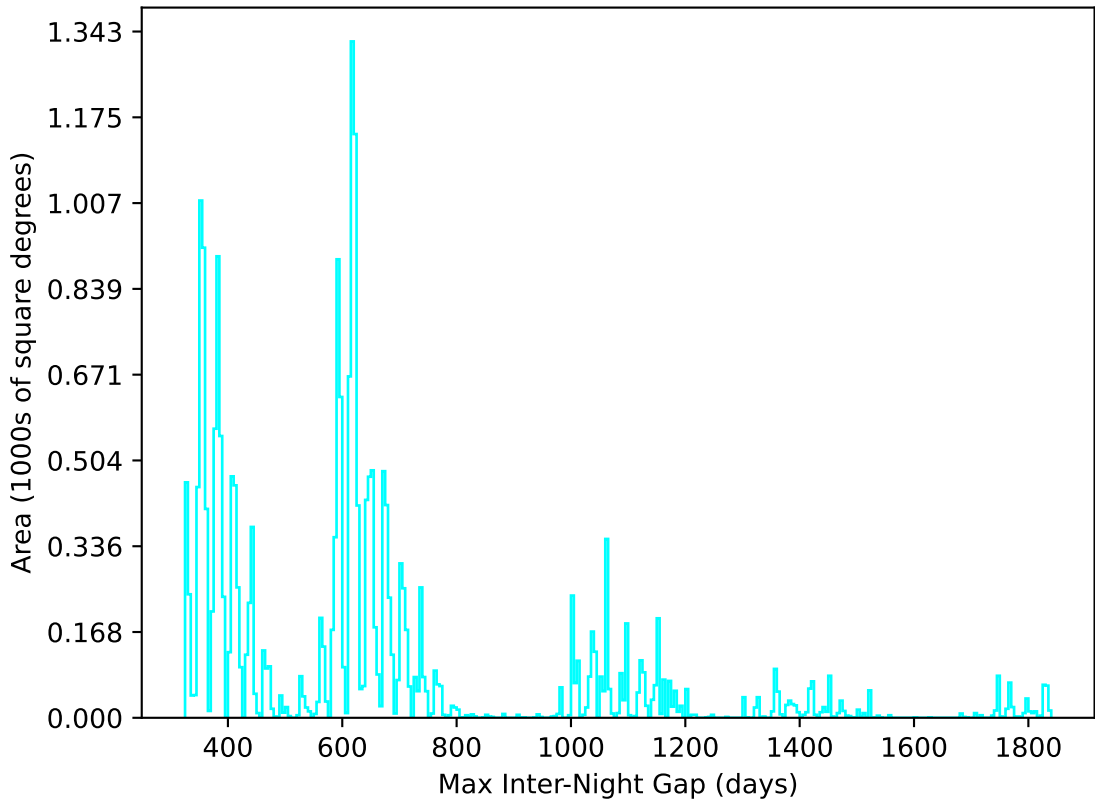
too_elab_r64_d3_gz_v3.4_10yrs All sky u band: Max Inter-Night Gap
