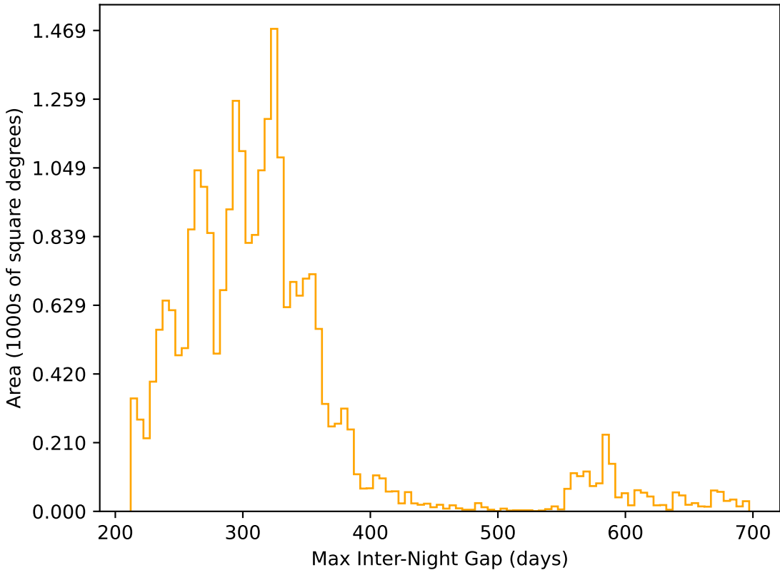
too_elab_r64_d3_gz_v3.4_10yrs All sky r band: Max Inter-Night Gap
