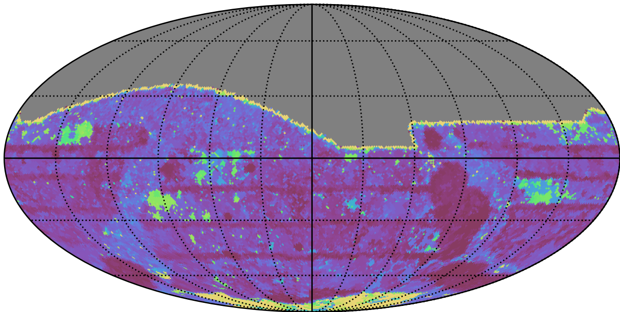
too_elab_r64_d3_gz_v3.4_10yrs All sky i band: Max Inter-Night Gap
