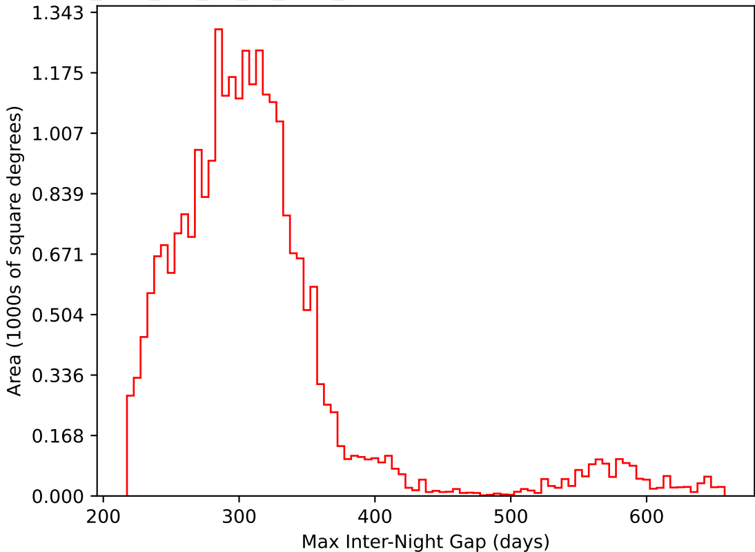
too_elab_r64_d3_gz_v3.4_10yrs All sky i band: Max Inter-Night Gap
