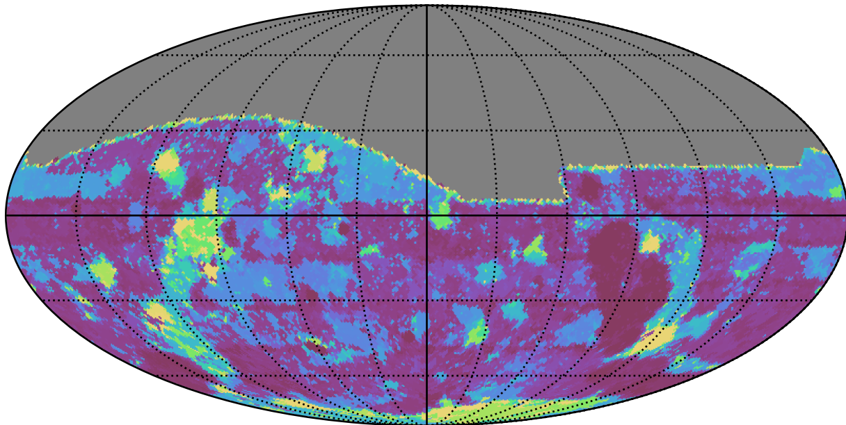
too_elab_r64_d3_gz_v3.4_10yrs All sky g band: Max Inter-Night Gap
