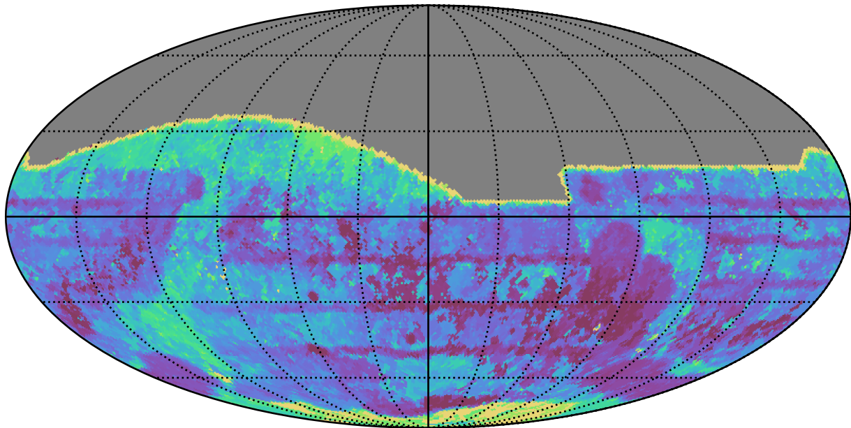
too_elab_r64_d3_gz_v3.4_10yrs All sky all bands: Max Inter-Night Gap
