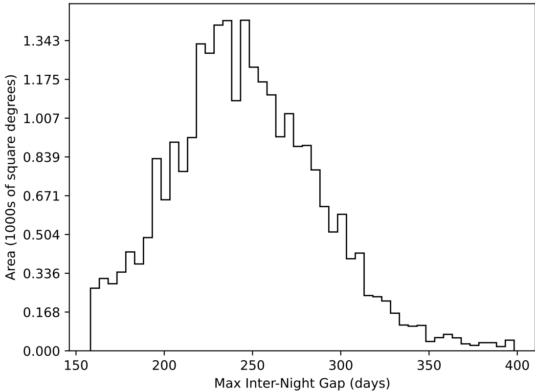
too_elab_r64_d3_gz_v3.4_10yrs All sky all bands: Max Inter-Night Gap
