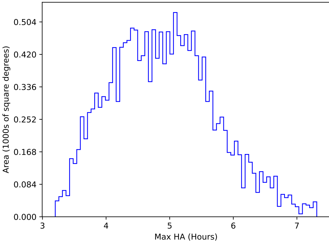
too_elab_r64_d3_gz_v3.4_10yrs WFD z band: Max HA
