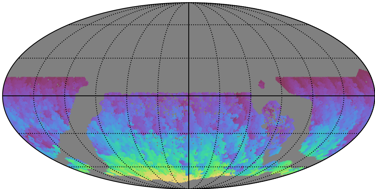
too_elab_r64_d3_gz_v3.4_10yrs WFD y band: Max HA
