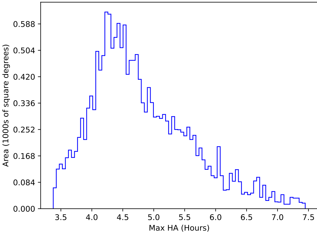
too_elab_r64_d3_gz_v3.4_10yrs WFD y band: Max HA
