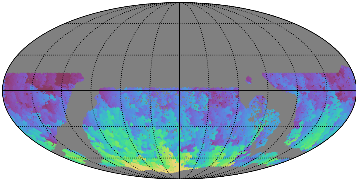
too_elab_r64_d3_gz_v3.4_10yrs WFD u band: Max HA
