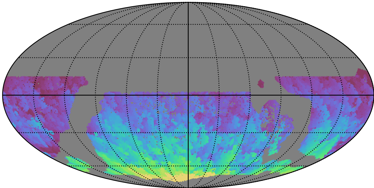
too_elab_r64_d3_gz_v3.4_10yrs WFD r band: Max HA
