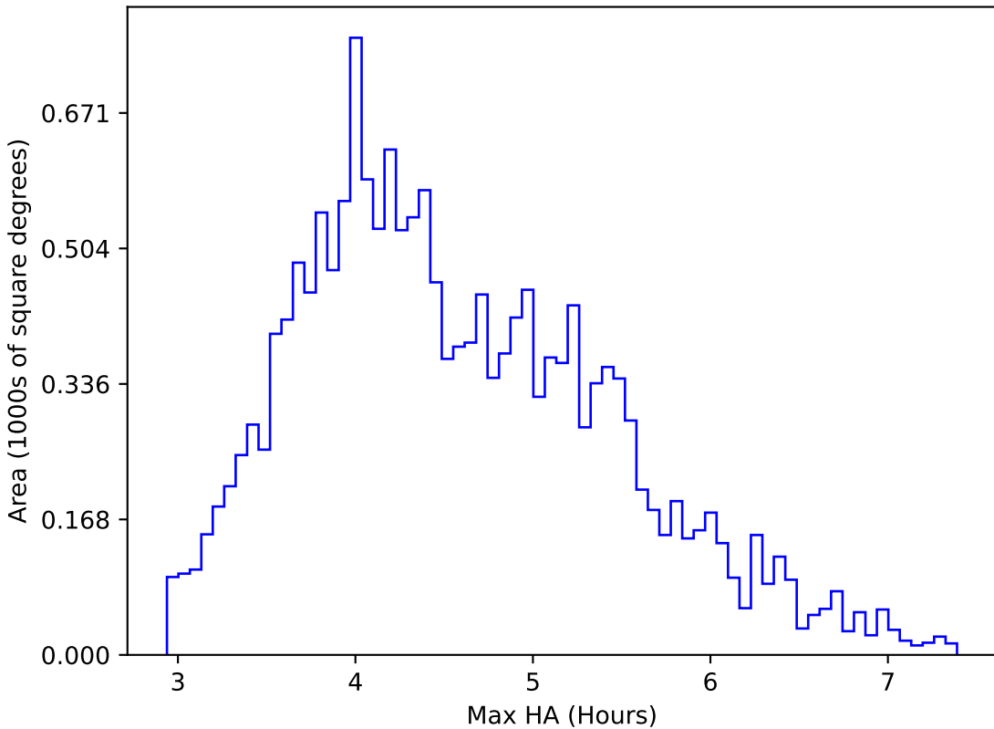
too_elab_r64_d3_gz_v3.4_10yrs WFD r band: Max HA
