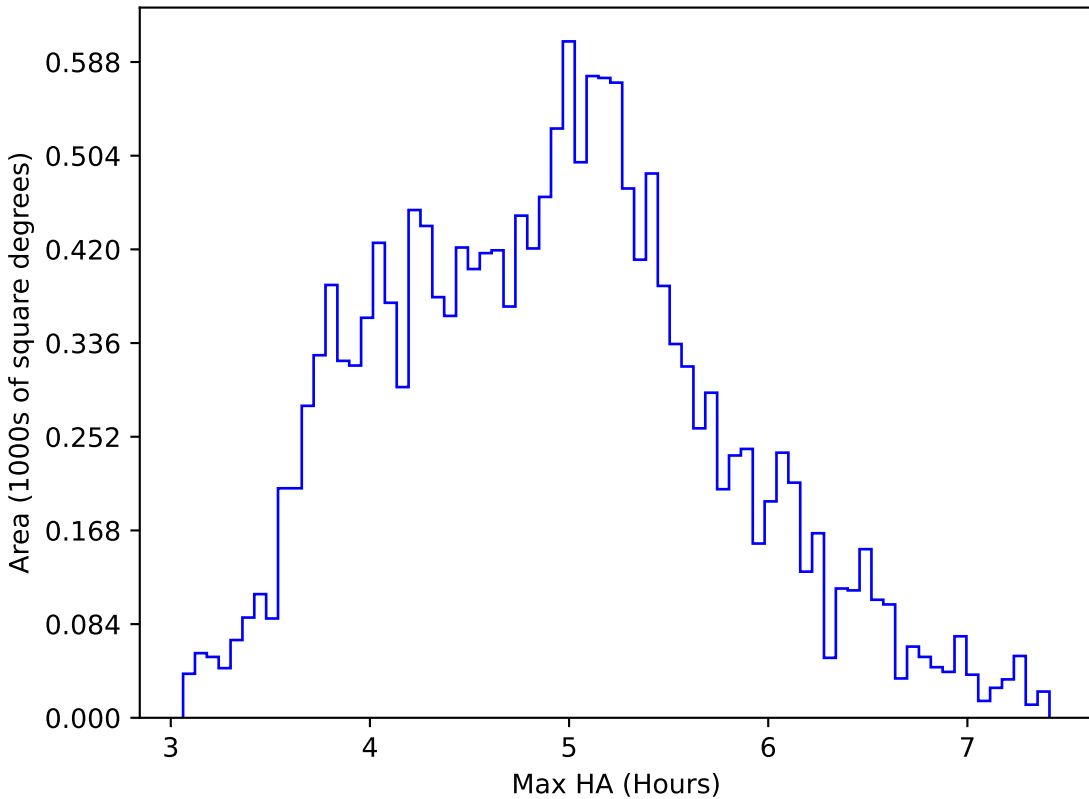
too_elab_r64_d3_gz_v3.4_10yrs WFD i band: Max HA
