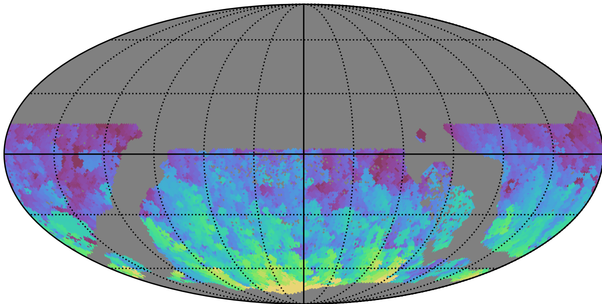
too_elab_r64_d3_gz_v3.4_10yrs WFD g band: Max HA
