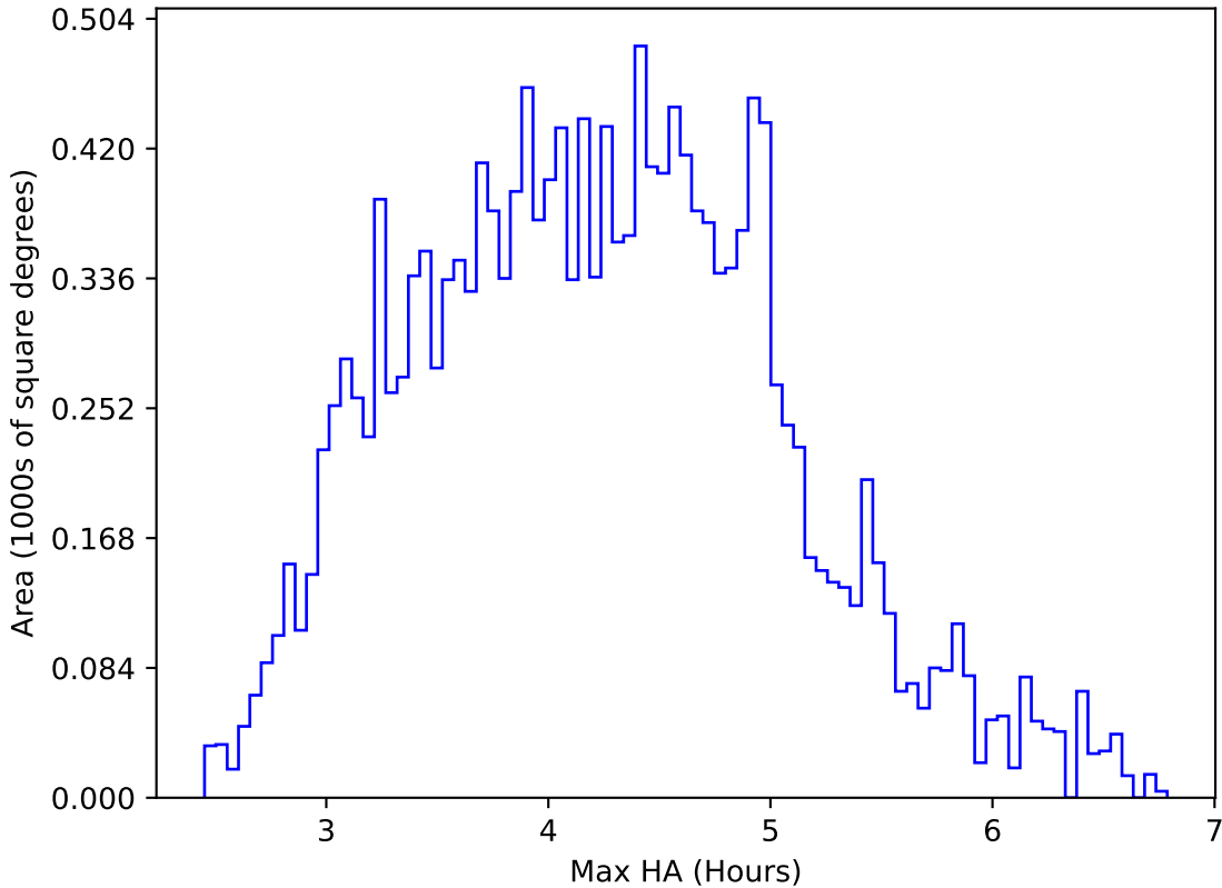
too_elab_r64_d3_gz_v3.4_10yrs WFD g band: Max HA
