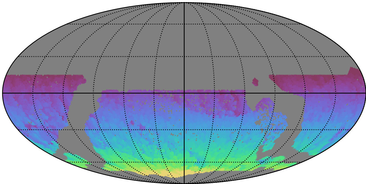
too_elab_r64_d3_gz_v3.4_10yrs WFD all bands: Max HA
