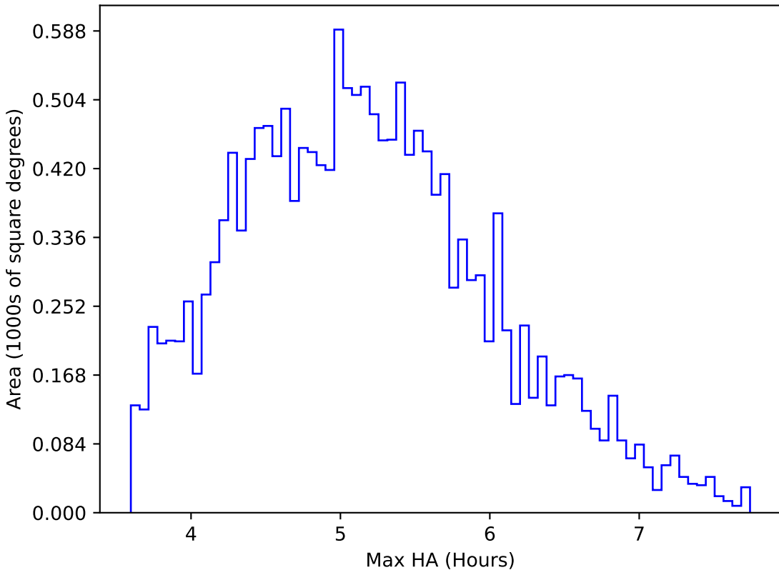
too_elab_r64_d3_gz_v3.4_10yrs WFD all bands: Max HA
