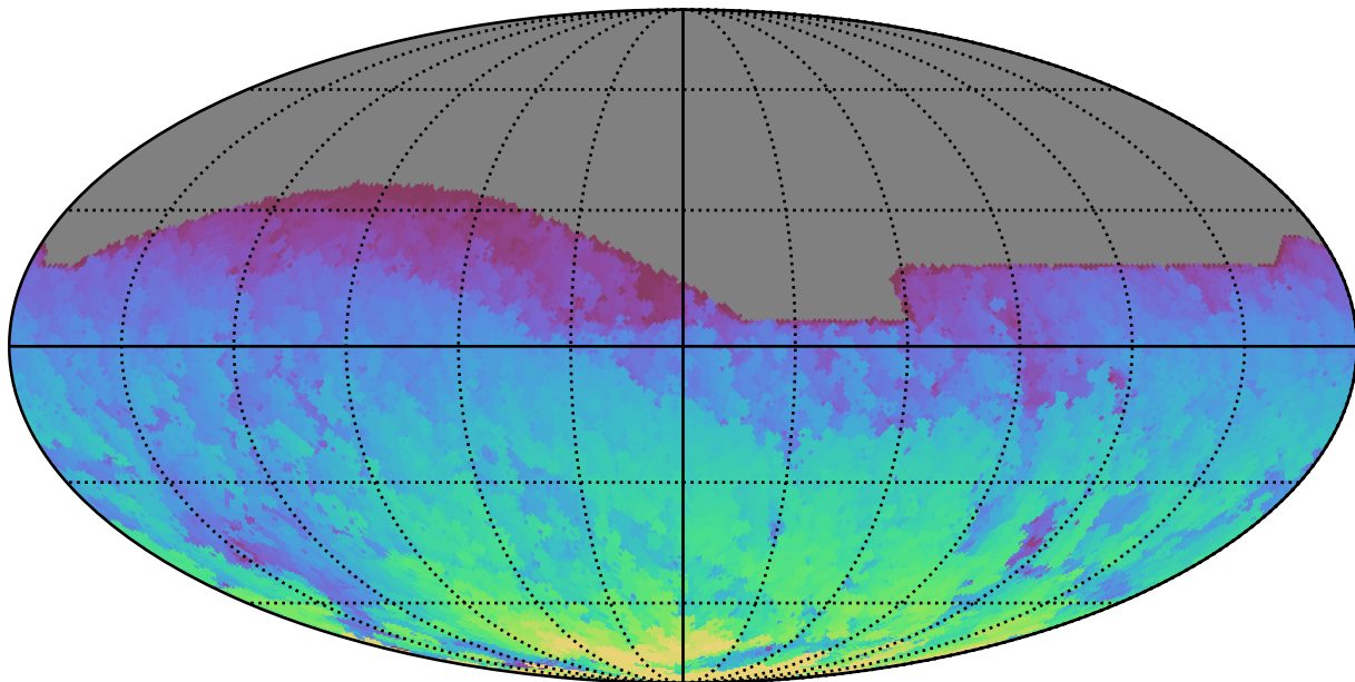
too_elab_r64_d3_gz_v3.4_10yrs All sky z band: Max HA
