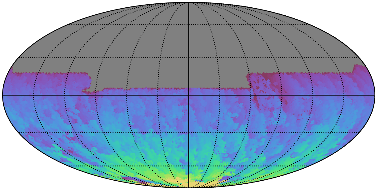
too_elab_r64_d3_gz_v3.4_10yrs All sky y band: Max HA
